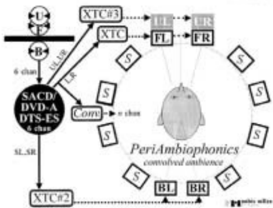
Fig. 7 Periambiophonics Provides An Elevated Stage
