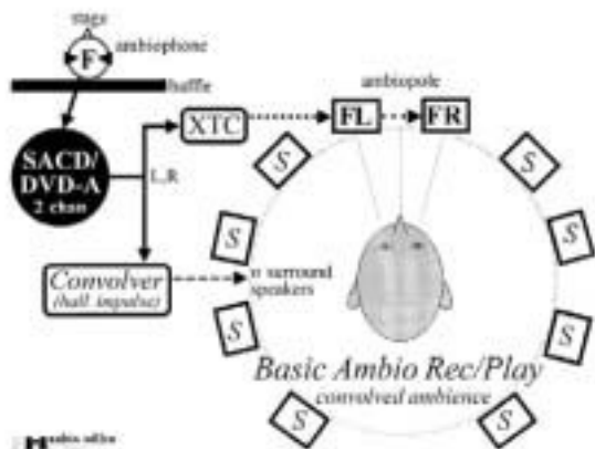
Fig. 3. Two Channel Ambiophonic System
