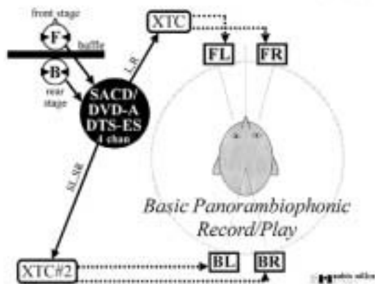
Fig. 5 Panorambiophonics Delivers Full Circle Localization via 4 Channels and Speakers
